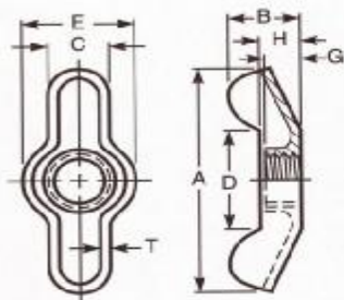
STYLE 2 (LOW WING)
